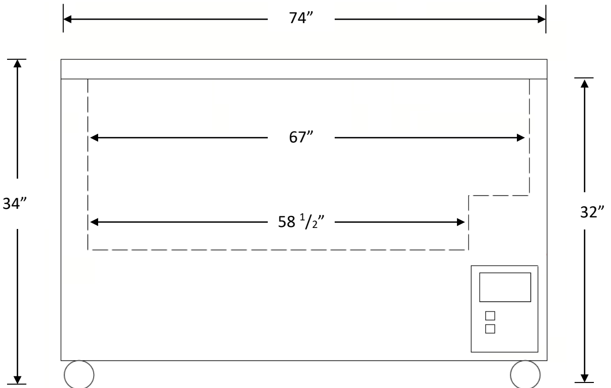
Chest Freezer Front View
